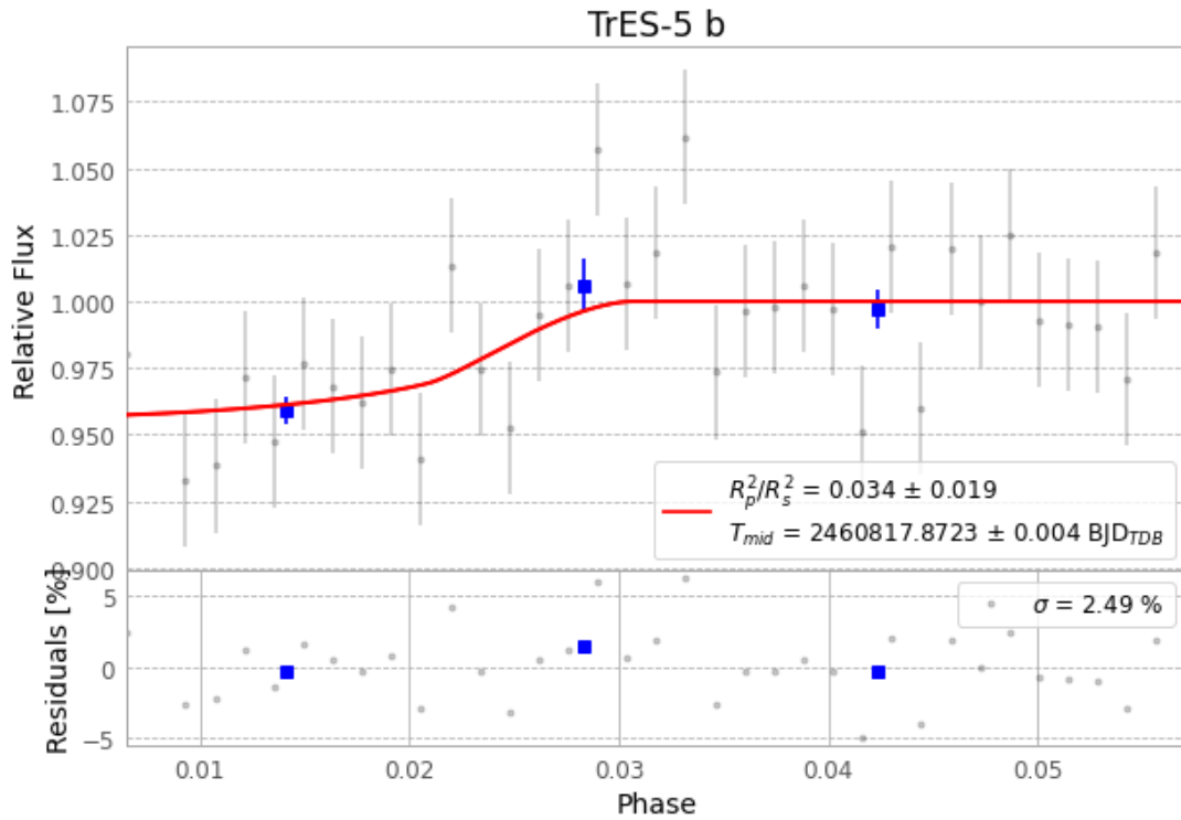
Figure 1 — FinalLightCurve_TrES-5 b_2025-05-22.png (SHA-256 a4c693fbff2c947f...)
