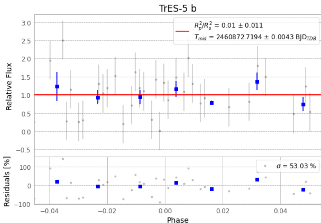
Figure 1 — FinalLightCurve_TrES-5 b_2025-07-15.png (SHA-256 35b72f3897f5b466...)
