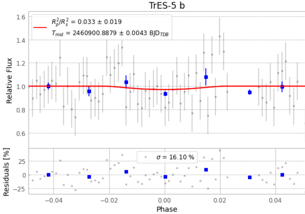
Figure 1 — FinalLightCurve_TrES-5 b_2025-08-13.png (SHA-256 15db9dd2ae89e637...)
