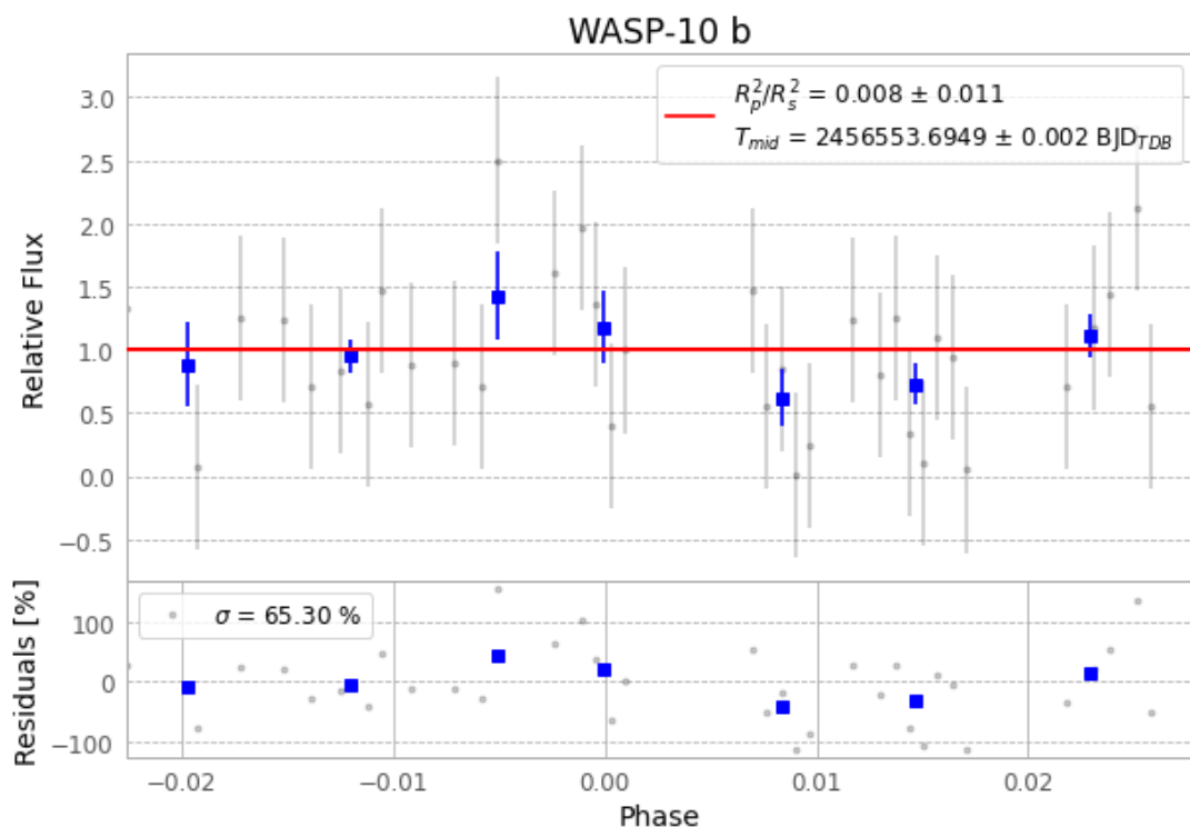
Figure 1 — FinalLightCurve_WASP-10 b_2013-09-17.png (SHA-256 7309ef7952559fa2...)
