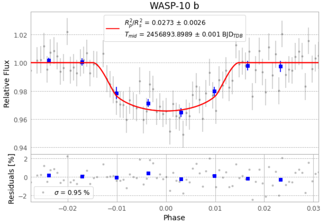
Figure 1 — FinalLightCurve_WASP-10 b_2014-08-24.png (SHA-256 5644d80602af7d08...)
