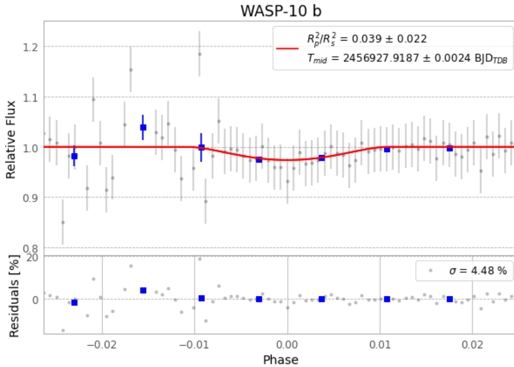
Figure 1 — FinalLightCurve_WASP-10 b_2014-09-27.png (SHA-256 e687fe87e7de8a5d...)
