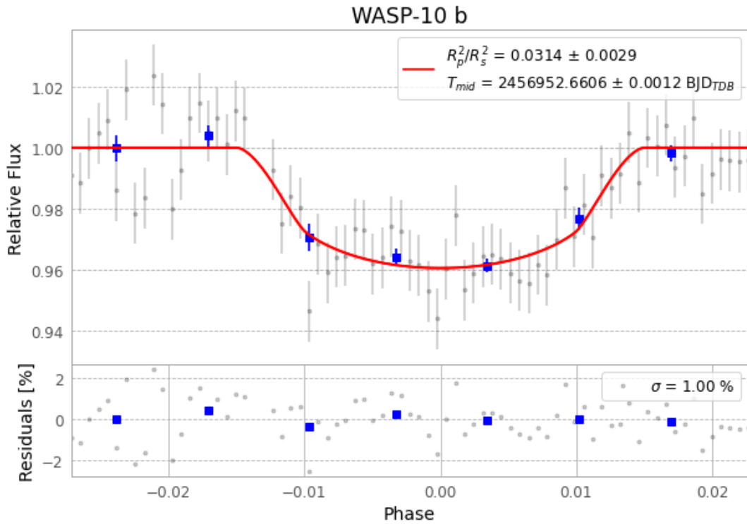
Figure 1 — FinalLightCurve_WASP-10 b_2014-10-21.png (SHA-256 c438b7f5f6a3c88d...)
