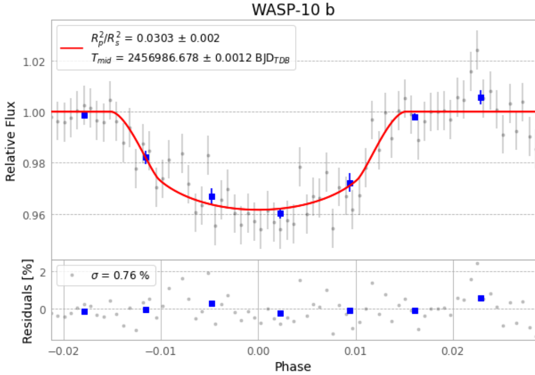
Figure 1 — FinalLightCurve_WASP-10 b_2014-11-24.png (SHA-256 919624565b9fb29e...)
