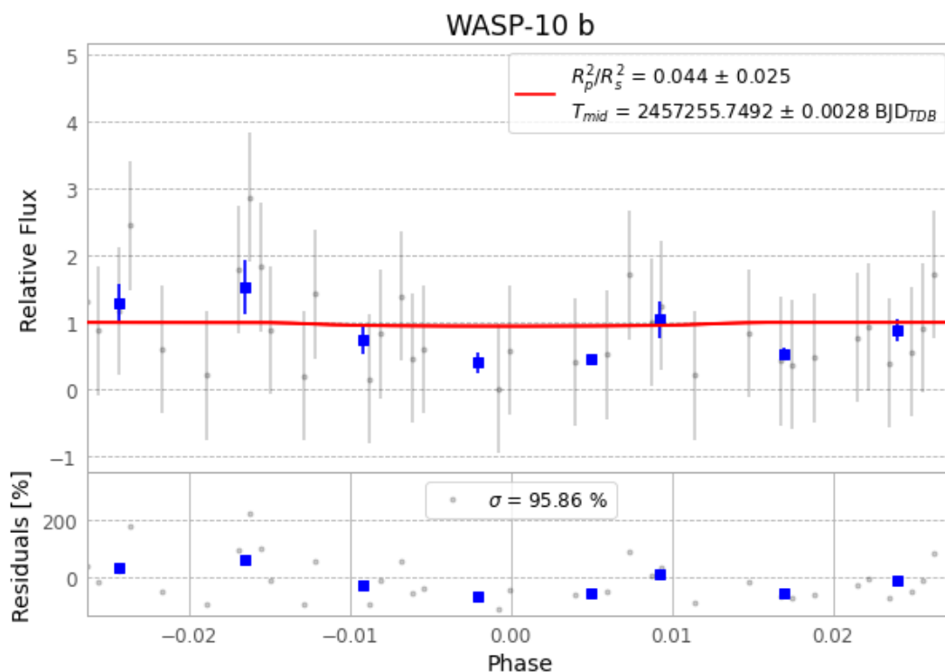
Figure 1 — FinalLightCurve_WASP-10 b_2015-08-20.png (SHA-256 874047aa7252b25b...)
