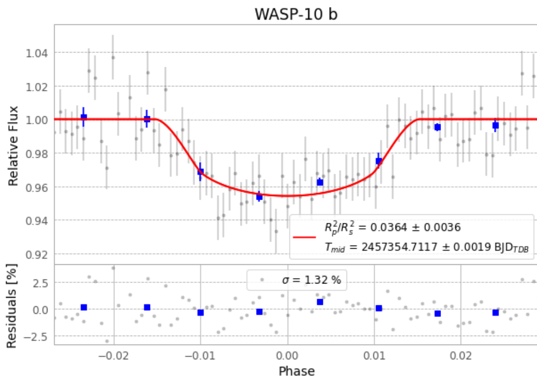
Figure 1 — FinalLightCurve_WASP-10 b_2015-11-27.png (SHA-256 301ad7f91243dfb8...)
