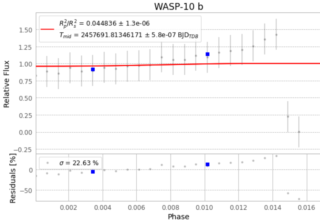
Figure 1 — FinalLightCurve_WASP-10 b_2016-10-30.png (SHA-256 1fad80e804b9c147...)
