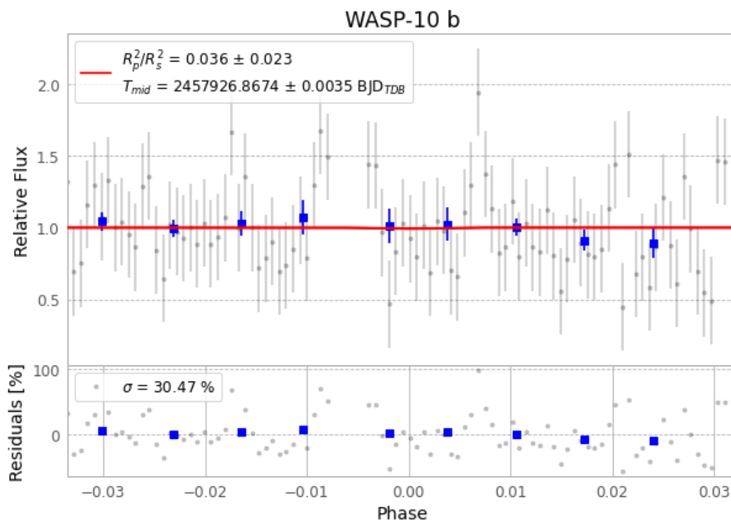
Figure 1 — FinalLightCurve_WASP-10 b_2017-06-21.png (SHA-256 2c2d0bf9b9fd40b2...)
