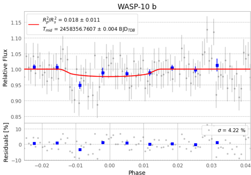
Figure 1 — FinalLightCurve_WASP-10 b_2018-08-25.png (SHA-256 b5a615d5d7747f56...)
