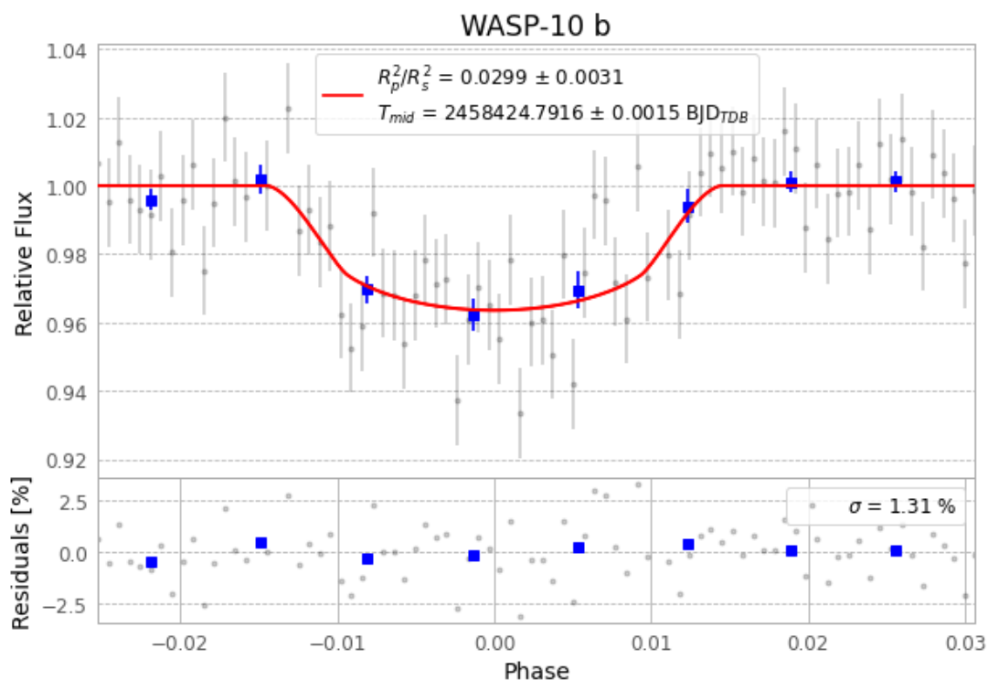
Figure 1 — FinalLightCurve_WASP-10 b_2018-11-01.png (SHA-256 73f5f18b7af2e7e1...)
