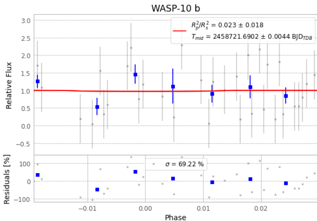
Figure 1 — FinalLightCurve_WASP-10 b_2019-08-25.png (SHA-256 58b6c030c1d416a9...)
