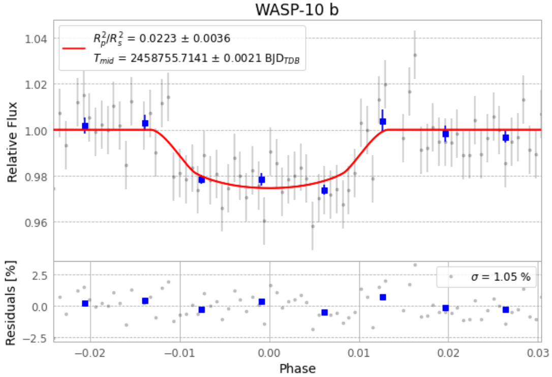
Figure 1 — FinalLightCurve_WASP-10 b_2019-09-28.png (SHA-256 886eeae4b7e97110...)
