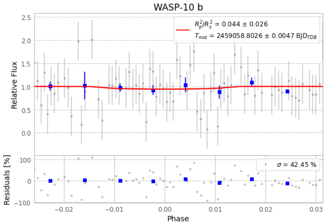
Figure 1 — FinalLightCurve_WASP-10 b_2020-07-27.png (SHA-256 cafb5f05c35e25f2...)
