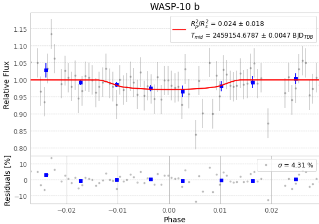
Figure 1 — FinalLightCurve_WASP-10 b_2020-10-31.png (SHA-256 cc4c890ee046fa84...)
