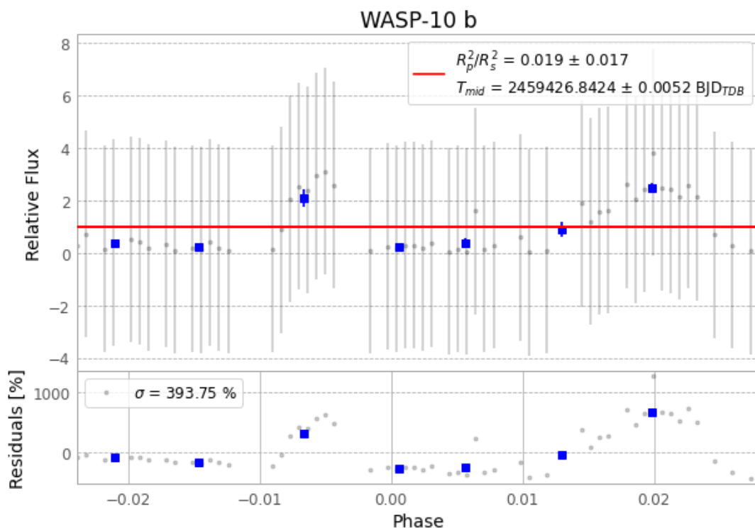
Figure 1 — FinalLightCurve_WASP-10 b_2021-07-30.png (SHA-256 ad7fb673c7f570b8...)
