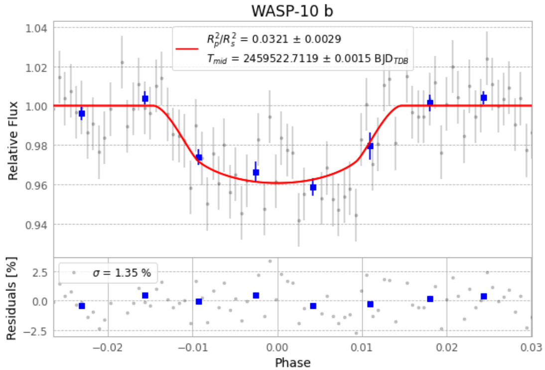
Figure 1 — FinalLightCurve_WASP-10 b_2021-11-03.png (SHA-256 170d8c88738cad34...)
