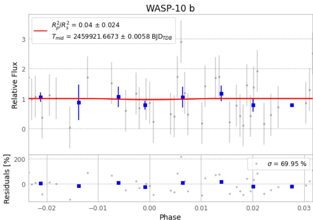
Figure 1 — FinalLightCurve_WASP-10 b_2022-12-07.png (SHA-256 7ddb431d719656eb...)
