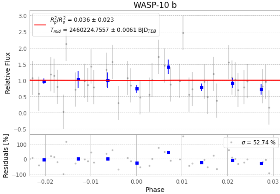
Figure 1 — FinalLightCurve_WASP-10 b_2023-10-06.png (SHA-256 e4f65e65438e73dd...)
