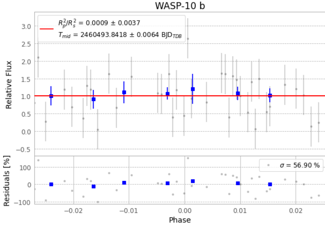
Figure 1 — FinalLightCurve_WASP-10 b_2024-07-01.png (SHA-256 021c84ba0b1c6717...)
