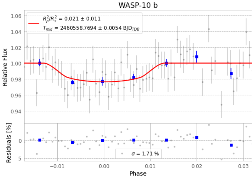
Figure 1 — FinalLightCurve_WASP-10 b_2024-09-04.png (SHA-256 ea4f4fe0292e3169...)
