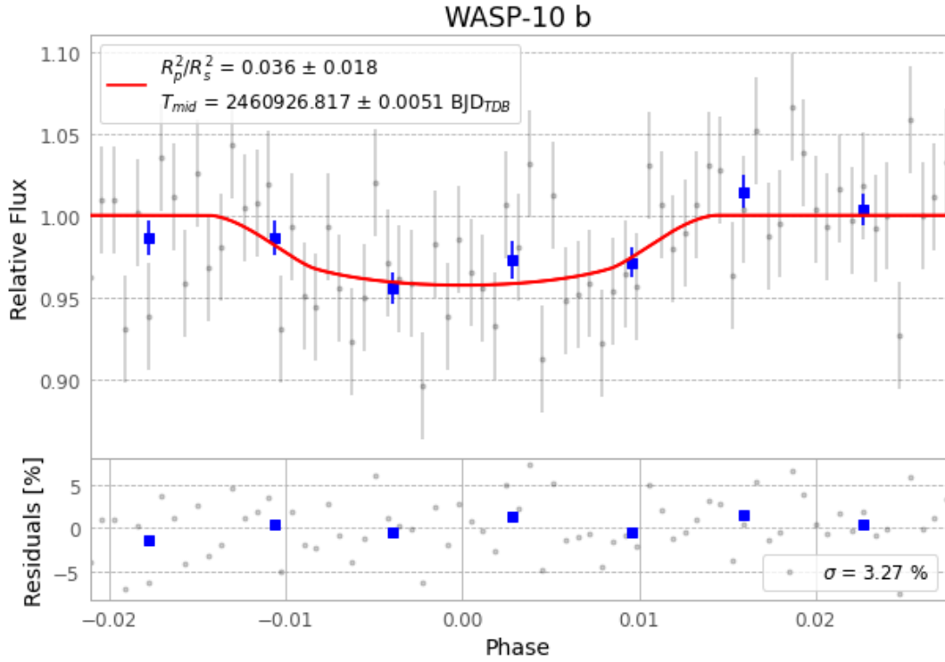
Figure 1 — FinalLightCurve_WASP-10 b_2025-09-07.png (SHA-256 16843080b6198a74...)
