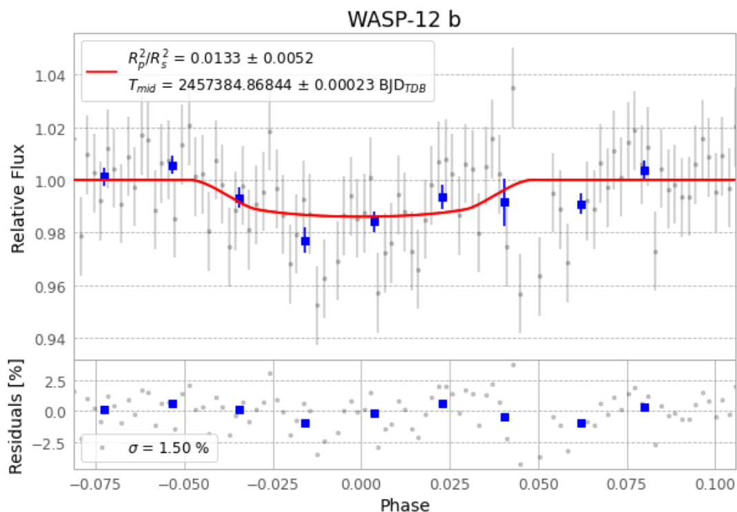
Figure 1 — FinalLightCurve_WASP-12 b_2015-12-27.png (SHA-256 8473757506b4bbee...)
