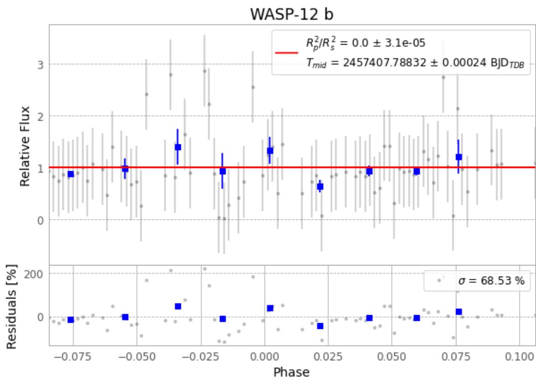
Figure 1 — FinalLightCurve_WASP-12 b_2016-01-19.png (SHA-256 48b5326eb0e19a64...)
