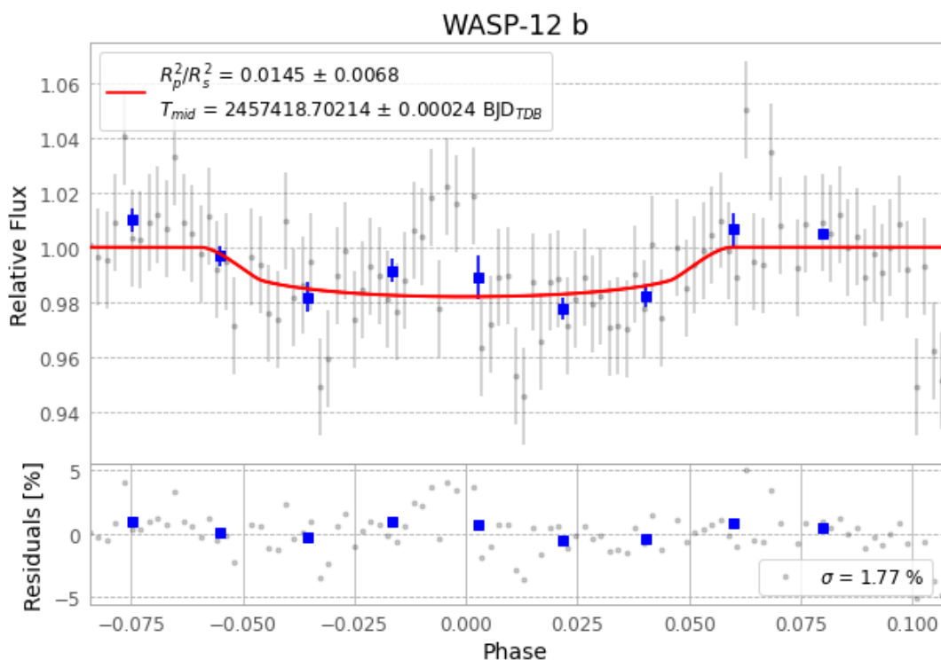
Figure 1 — FinalLightCurve_WASP-12 b_2016-01-30.png (SHA-256 221dcb0658002f9f...)
