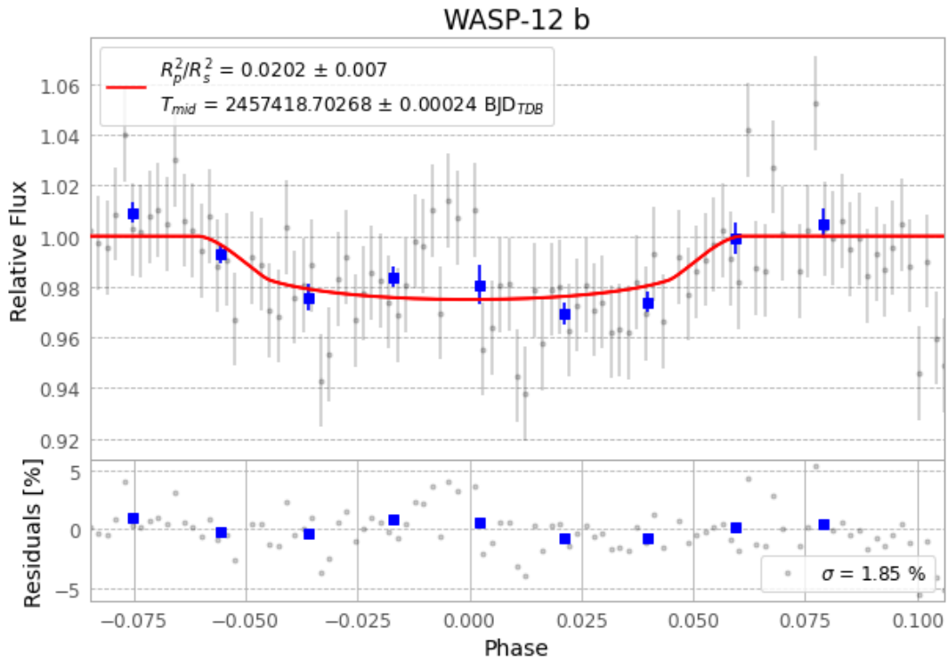
Figure 1 — FinalLightCurve_WASP-12 b_2016-01-30.png (SHA-256 8ef2f8b52128e5bd...)
