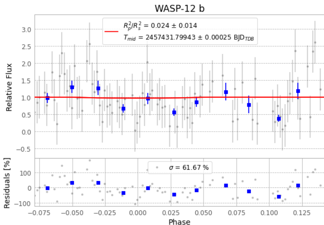
Figure 1 — FinalLightCurve_WASP-12 b_2016-02-12.png (SHA-256 466fd5de50ee806e...)
