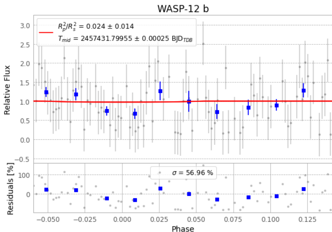
Figure 1 — FinalLightCurve_WASP-12 b_2016-02-12.png (SHA-256 88d593512e223ead...)
