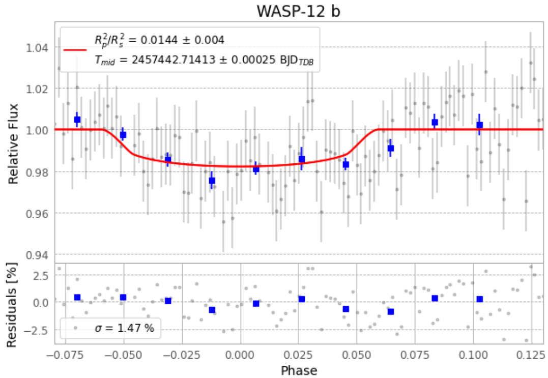
Figure 1 — FinalLightCurve_WASP-12 b_2016-02-23.png (SHA-256 281245d28b6a25c7...)
