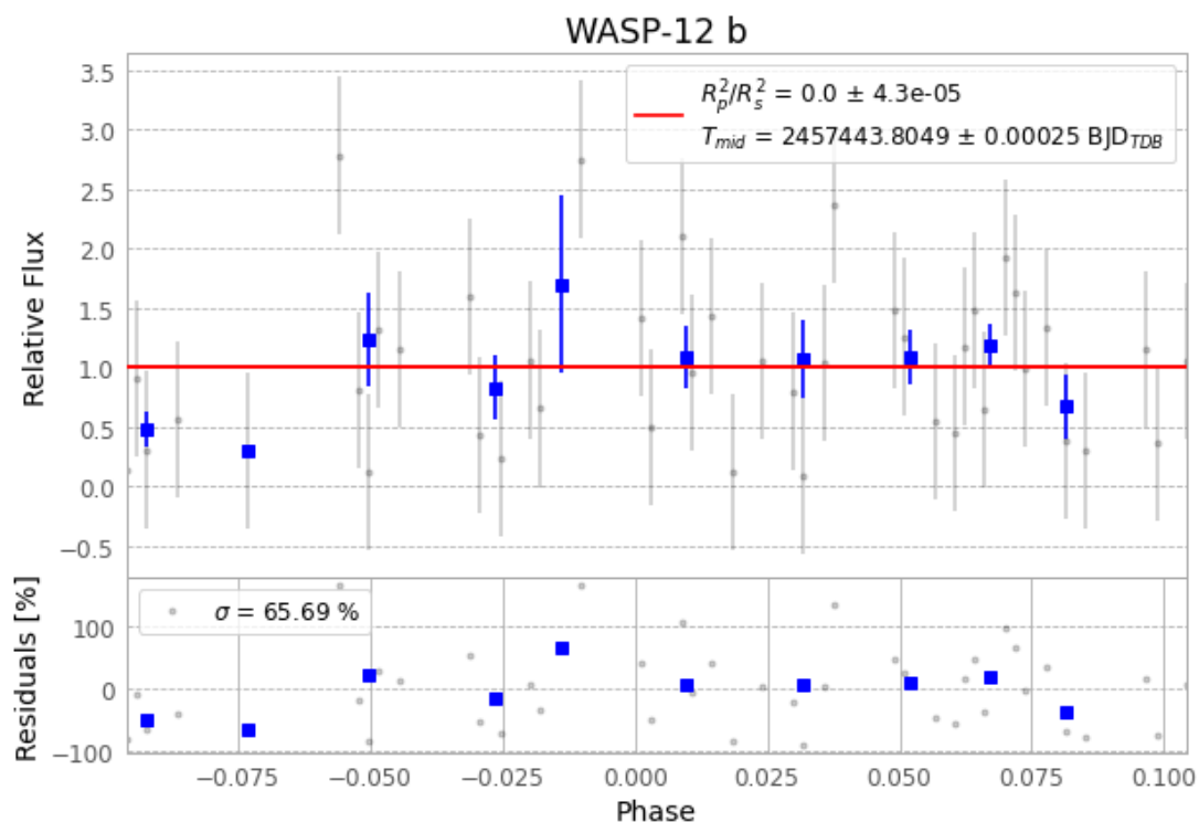
Figure 1 — FinalLightCurve_WASP-12 b_2016-02-24.png (SHA-256 7b52524eca02a035...)
