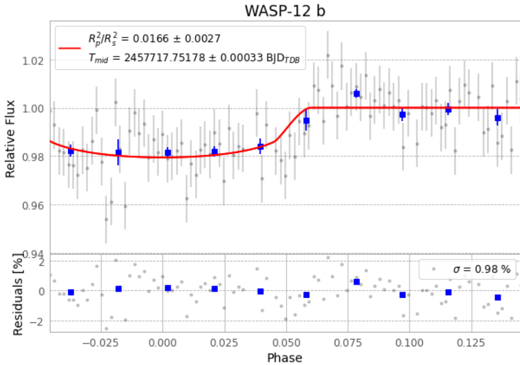
Figure 1 — FinalLightCurve_WASP-12 b_2016-11-24.png (SHA-256 9181af65de06a0f0...)
