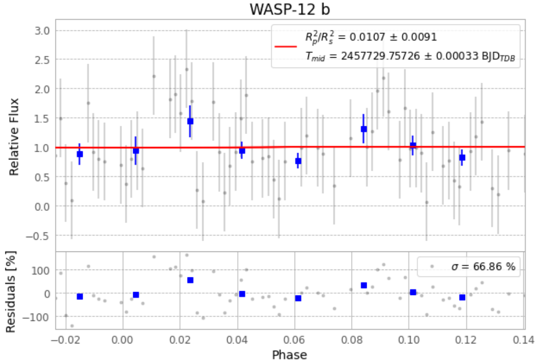
Figure 1 — FinalLightCurve_WASP-12 b_2016-12-06.png (SHA-256 beeb5ab829dd5c50...)
