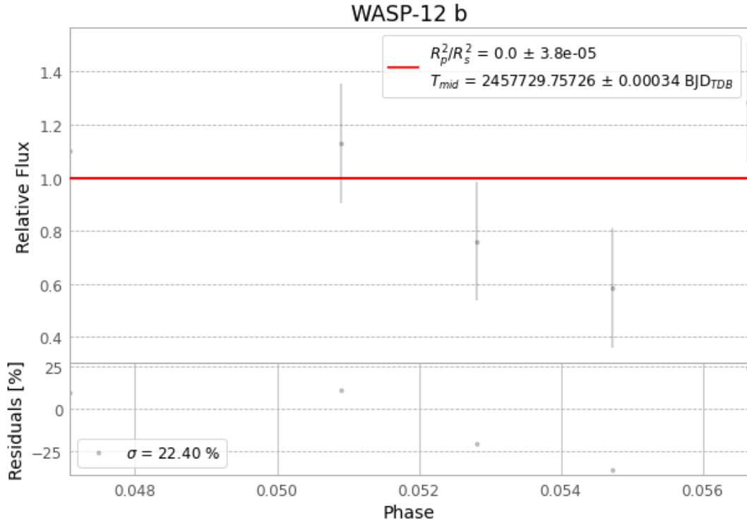
Figure 1 — FinalLightCurve_WASP-12 b_2016-12-07.png (SHA-256 f3b4f2fba6dd3d64...)
