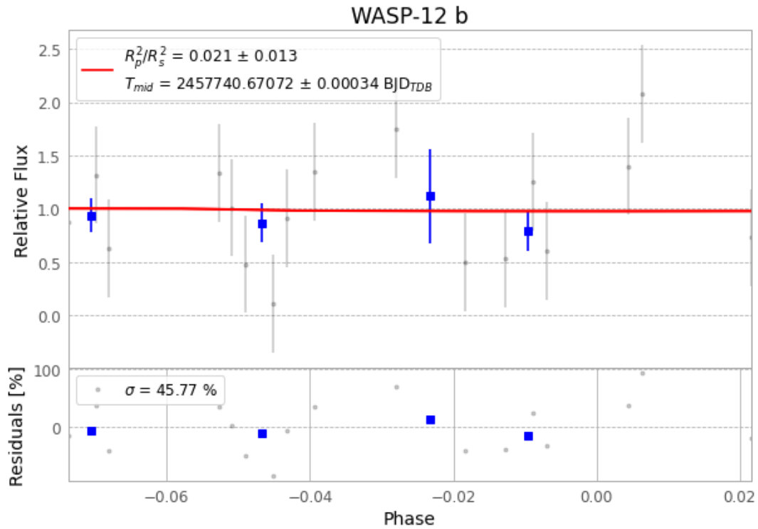
Figure 1 — FinalLightCurve_WASP-12 b_2016-12-17.png (SHA-256 631c82ea63a760ca...)
