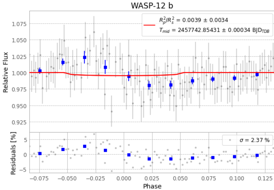
Figure 1 — FinalLightCurve_WASP-12 b_2016-12-19.png (SHA-256 7d57be292e46319e...)
