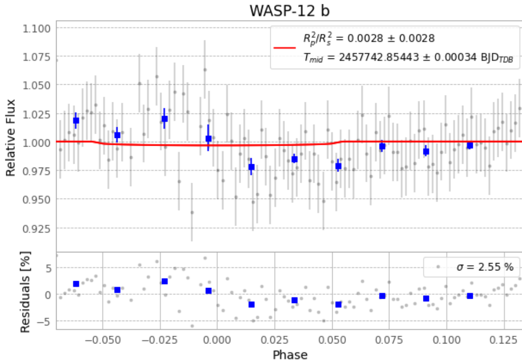
Figure 1 — FinalLightCurve_WASP-12 b_2016-12-19.png (SHA-256 34b6f61f95bc96cf...)
