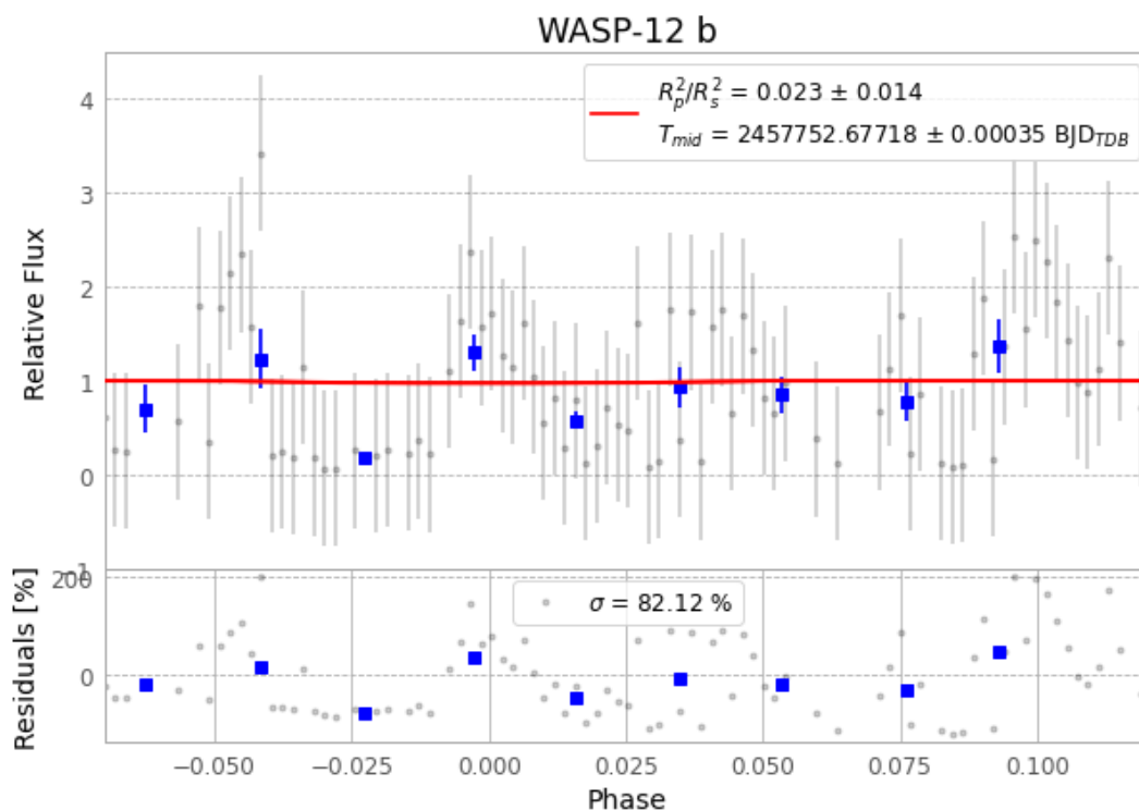
Figure 1 — FinalLightCurve_WASP-12 b_2016-12-29.png (SHA-256 2c6e3d3a22e44af1...)
