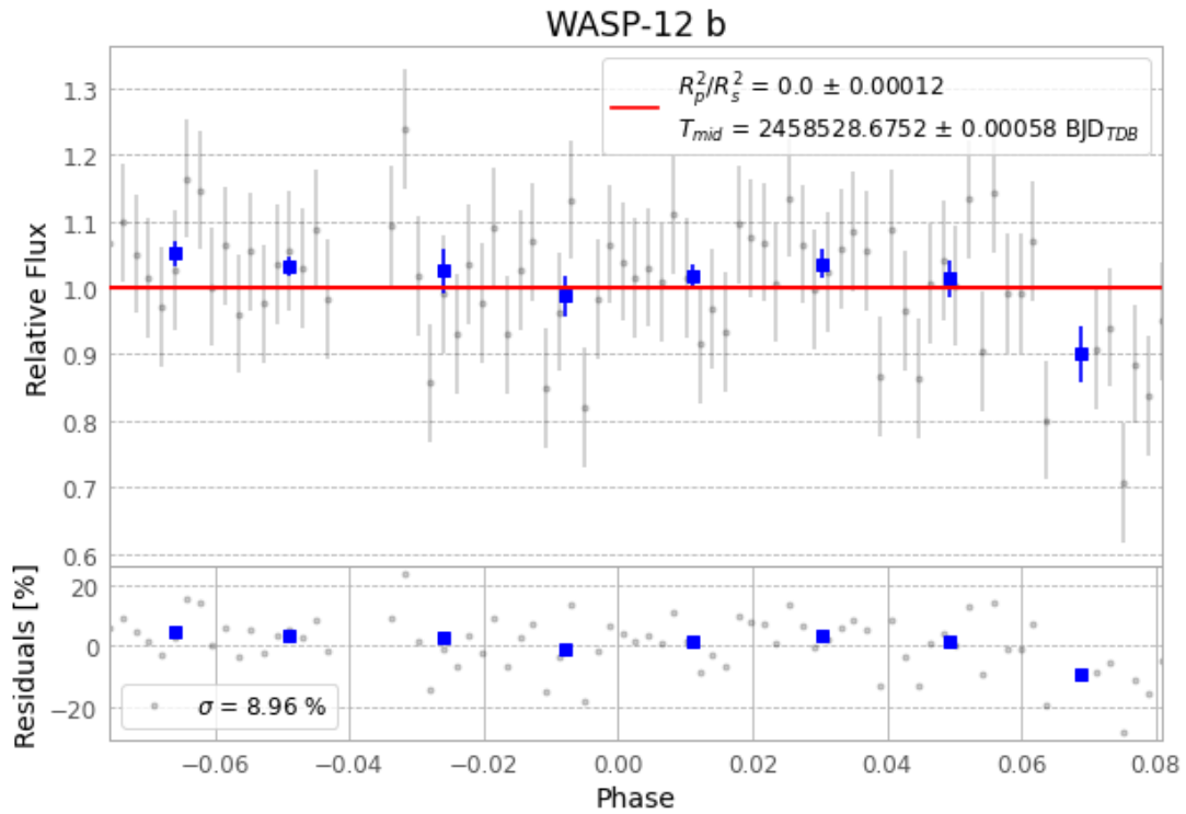
Figure 1 — FinalLightCurve_WASP-12 b_2019-02-13.png (SHA-256 70bf83f898363cec...)
