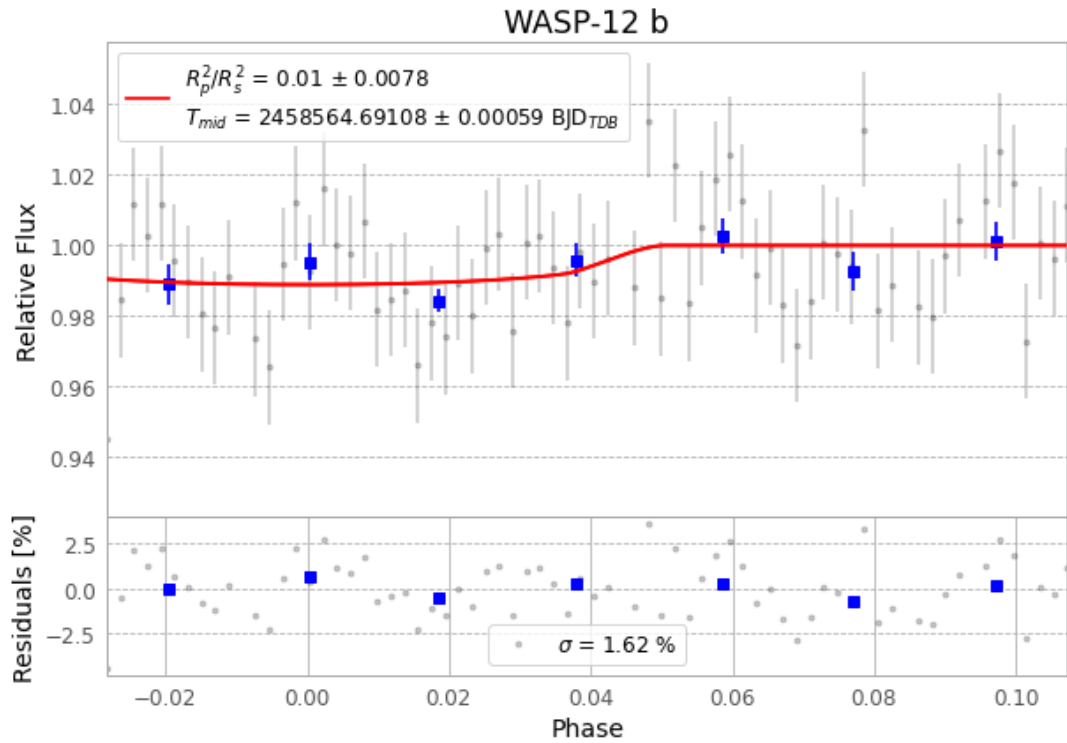
Figure 1 — FinalLightCurve_WASP-12 b_2019-03-21.png (SHA-256 7a46587bd8bed1d7...)
