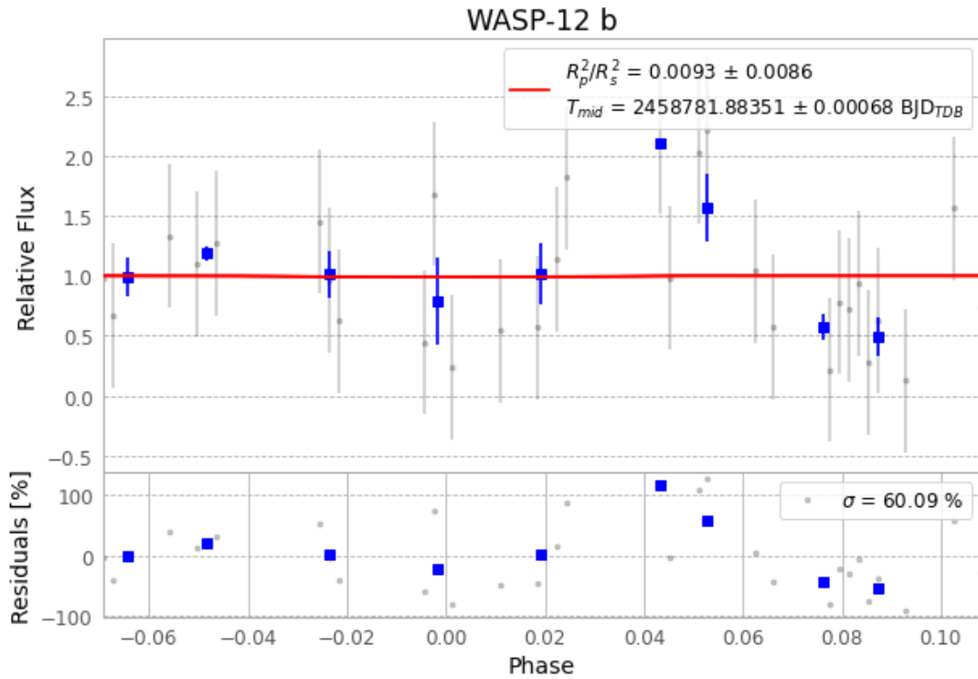
Figure 1 — FinalLightCurve_WASP-12 b_2019-10-25.png (SHA-256 d4a9eabd0bcb9874...)
