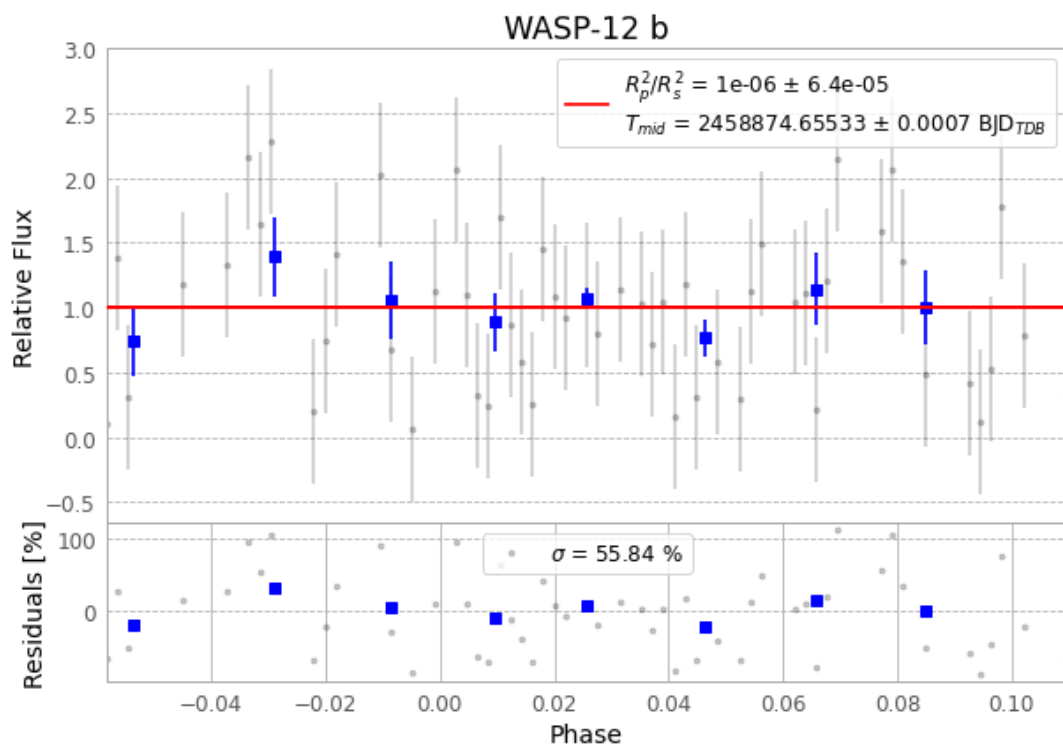
Figure 1 — FinalLightCurve_WASP-12 b_2020-01-25.png (SHA-256 b803c412548d1a32...)
