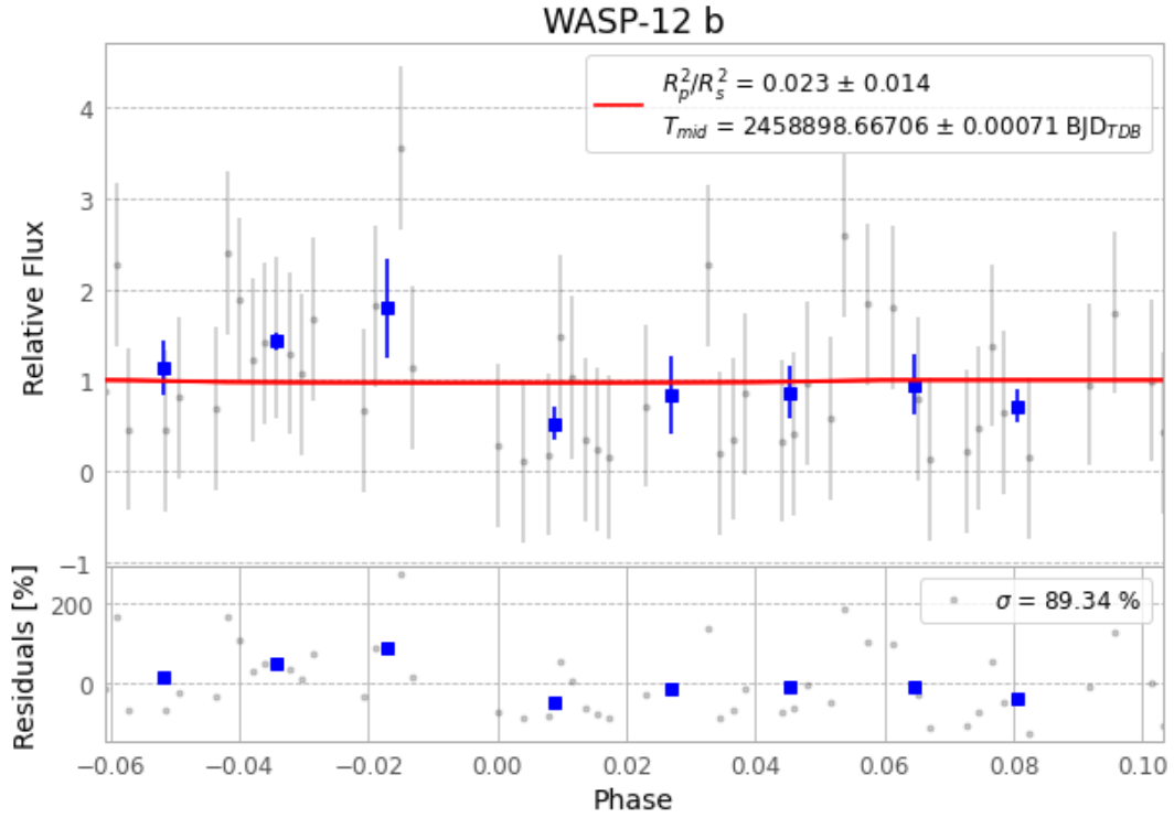
Figure 1 — FinalLightCurve_WASP-12 b_2020-02-18.png (SHA-256 c44cd0e50f1d716e...)
