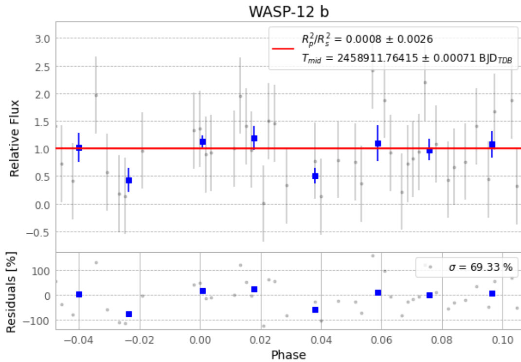
Figure 1 — FinalLightCurve_WASP-12 b_2020-03-02.png (SHA-256 2c8d743ee8a9bdae...)
