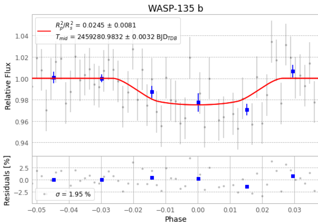
Figure 1 — FinalLightCurve_WASP-135 b_2021-03-07.png (SHA-256 97779d4d2615ceba...)
