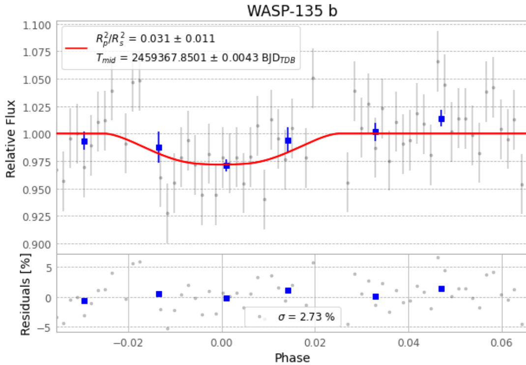
Figure 1 — FinalLightCurve_WASP-135 b_2021-06-02.png (SHA-256 9a04ad0bef3c97ab...)
