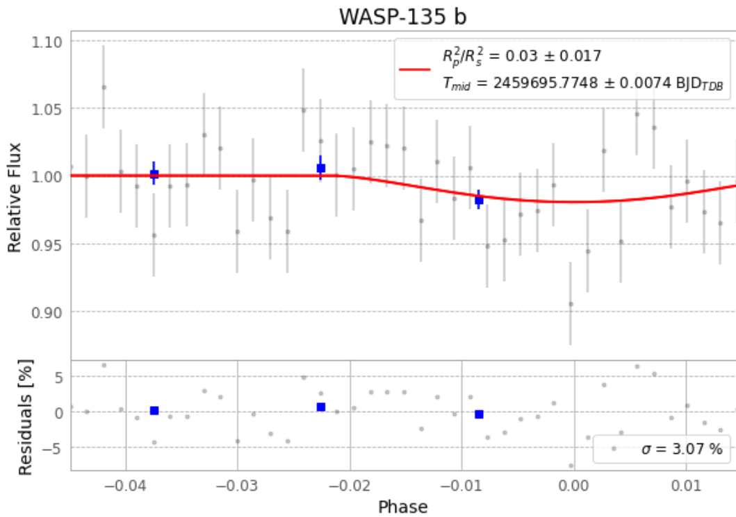
Figure 1 — FinalLightCurve_WASP-135 b_2022-04-25.png (SHA-256 345021d43efeb5b9...)
