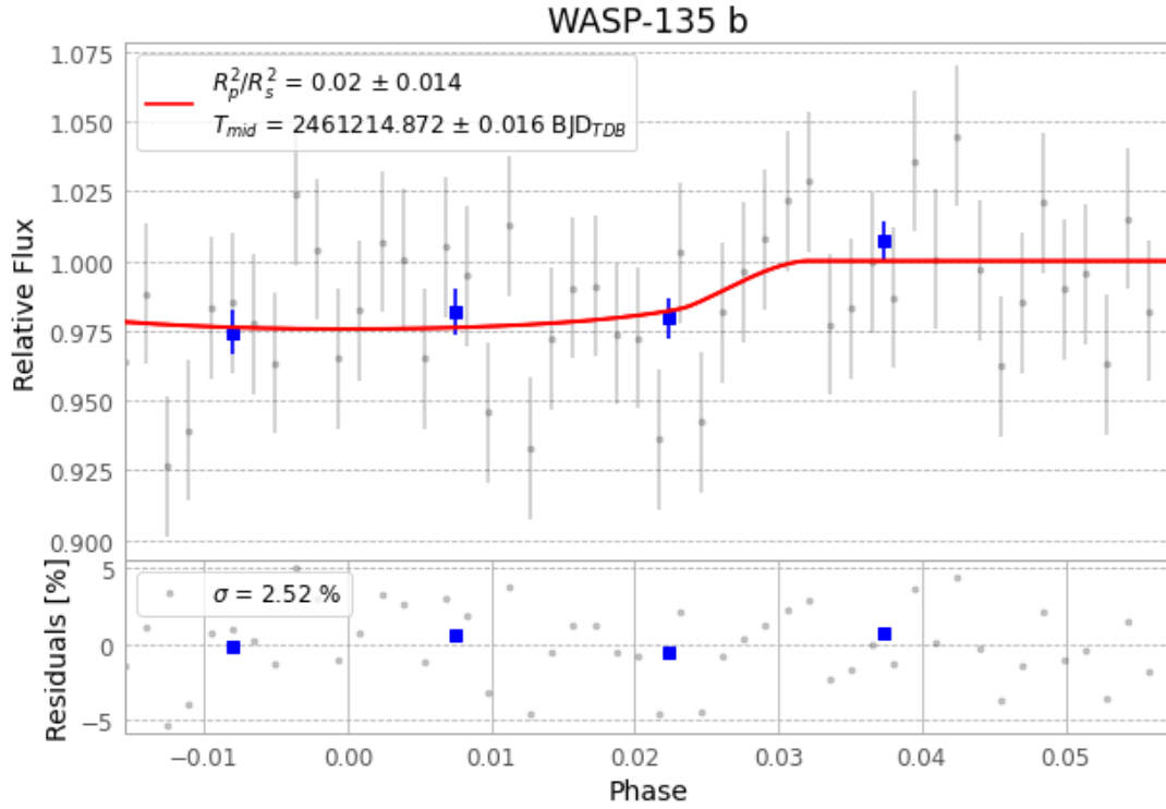
Figure 1 — FinalLightCurve_WASP-135 b_2026-06-23.png (SHA-256 01e8a0bc11d59205...)
